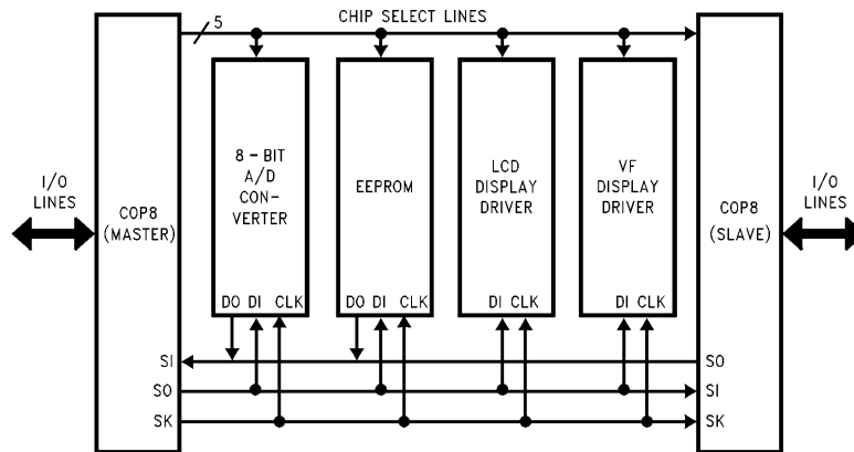
FIGURE 13. MICROWIRE/PLUS Application
